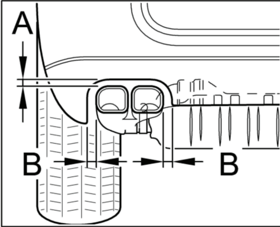
Fig. 53: Aligning tailpipes - Cayenne Turbo
